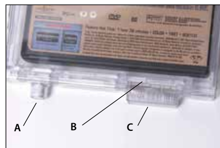
A. Security lock B. Security tab C. AM or RF Sensor
